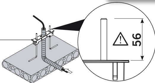
Accessory flange
