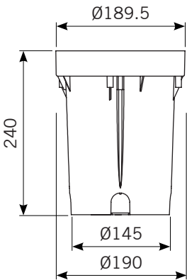
RECESS BOX
